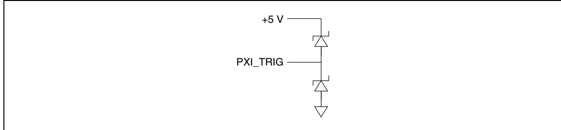
Figure 4-3. PXI Trigger Bus Termination
